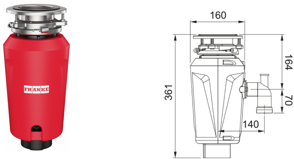
Food Waste Disposer SLIM 50 (1/2 HP)
